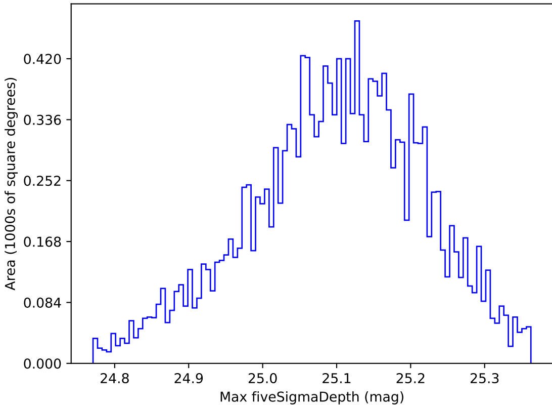
noroll_mjdp180_v3.4_10yrs WFD all bands: Max fiveSigmaDepth
