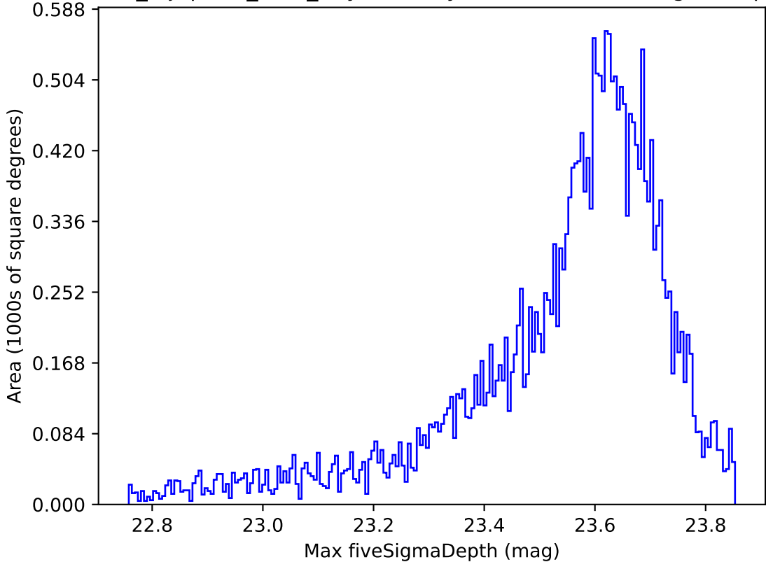
noroll_mjdp180_v3.4_10yrs All sky z band: Max fiveSigmaDepth
