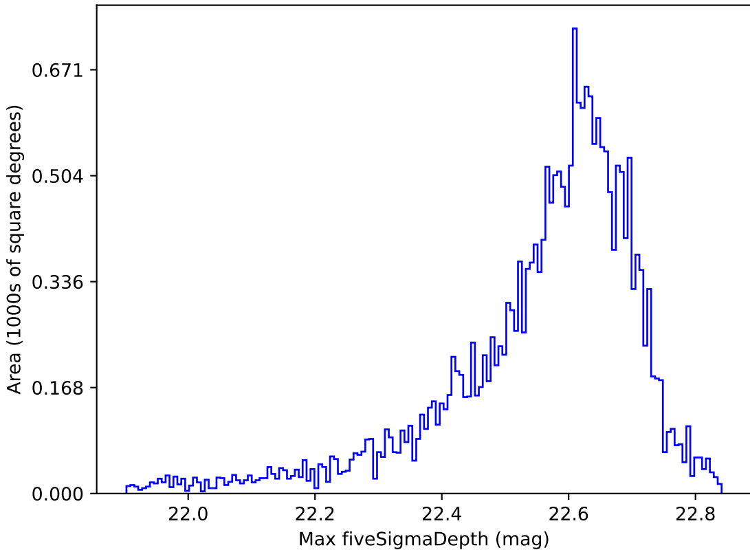
noroll_mjdp180_v3.4_10yrs All sky y band: Max fiveSigmaDepth
