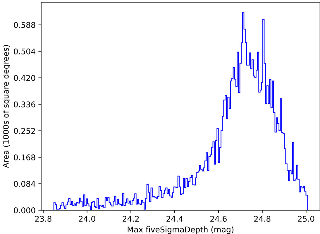
noroll_mjdp180_v3.4_10yrs All sky r band: Max fiveSigmaDepth
