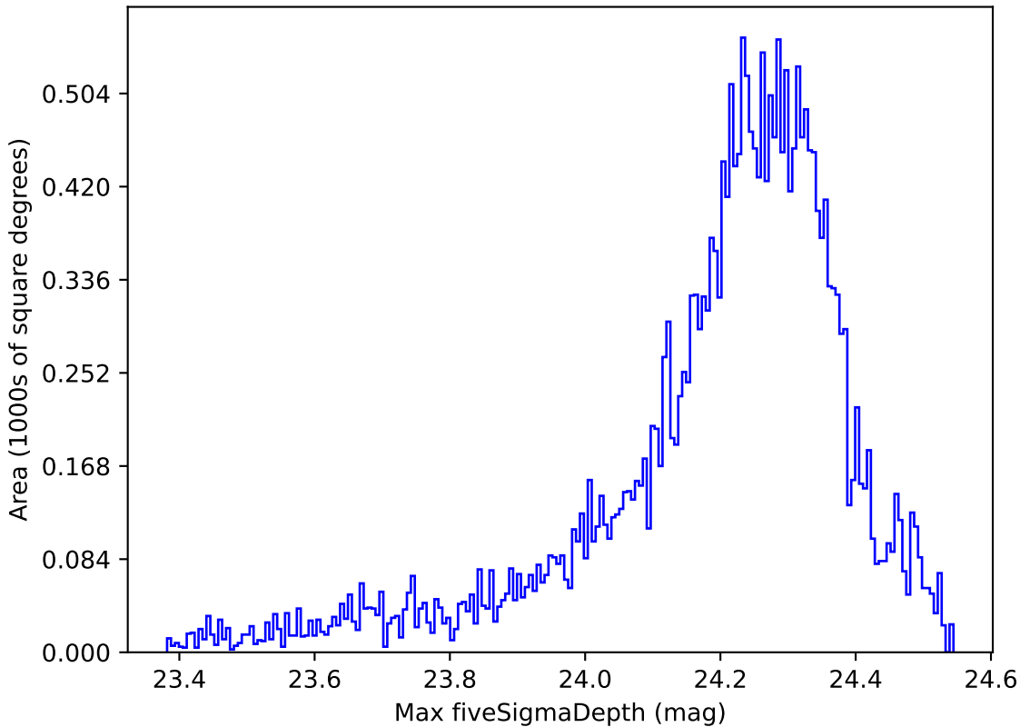
noroll_mjdp180_v3.4_10yrs All sky i band: Max fiveSigmaDepth
