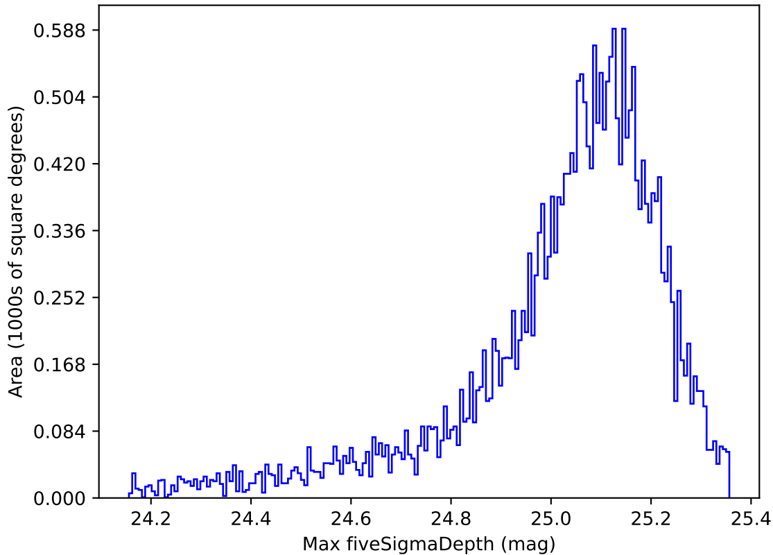
noroll_mjdp180_v3.4_10yrs All sky g band: Max fiveSigmaDepth
