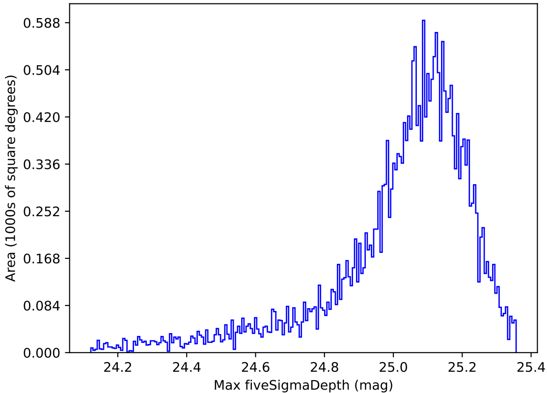
noroll_mjdp180_v3.4_10yrs All sky all bands: Max fiveSigmaDepth
