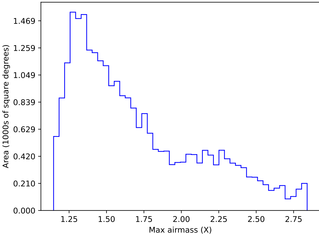
noroll_mjdp180_v3.4_10yrs Yr 1 z band: Max airmass
