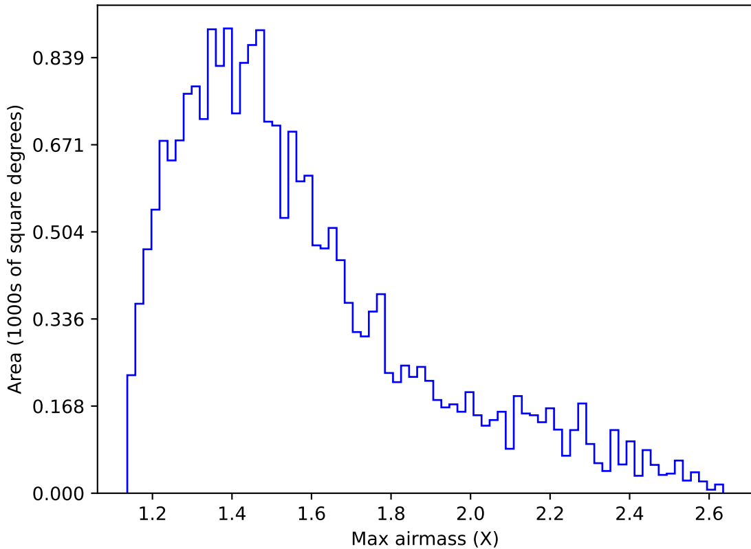
noroll_mjdp180_v3.4_10yrs Yr 1 y band: Max airmass
