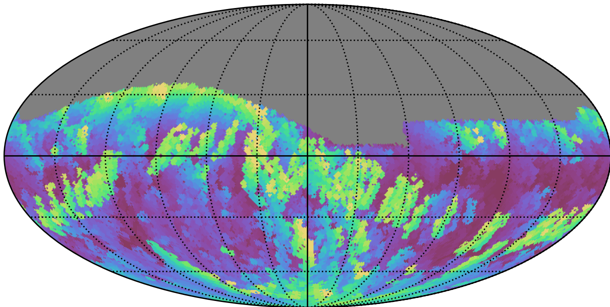
noroll_mjdp180_v3.4_10yrs Yr 1 r band: Max airmass
