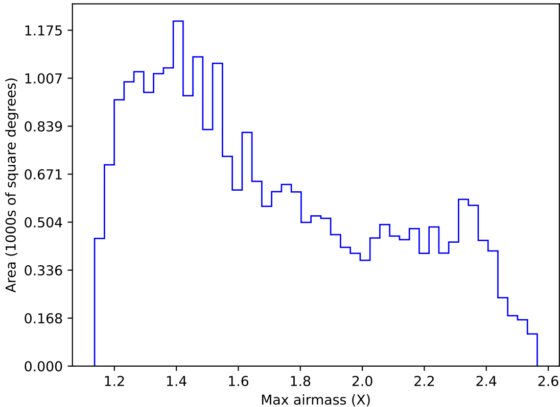
noroll_mjdp180_v3.4_10yrs Yr 1 r band: Max airmass
