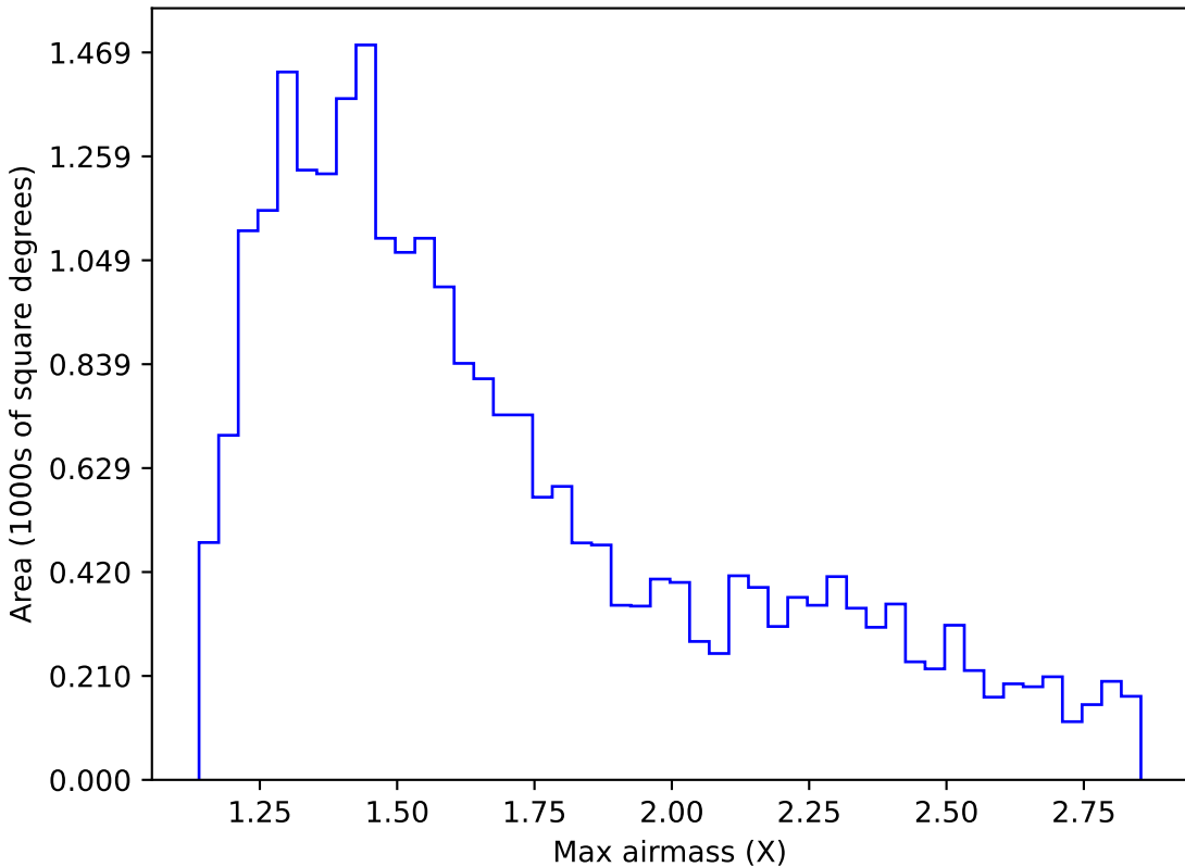
noroll_mjdp180_v3.4_10yrs Yr 1 i band: Max airmass
