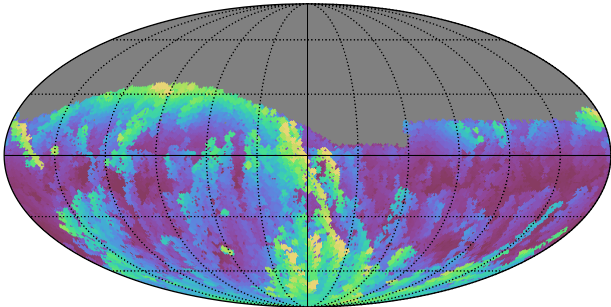
noroll_mjdp180_v3.4_10yrs Yr 1 g band: Max airmass
