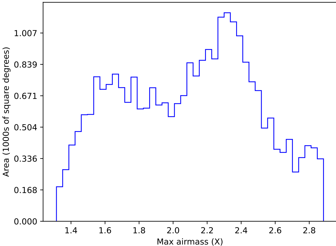
noroll_mjdp180_v3.4_10yrs Yr 1 all bands: Max airmass
