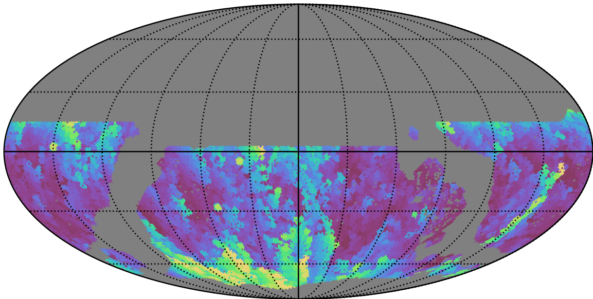
noroll_mjdp180_v3.4_10yrs WFD u band: Max airmass
