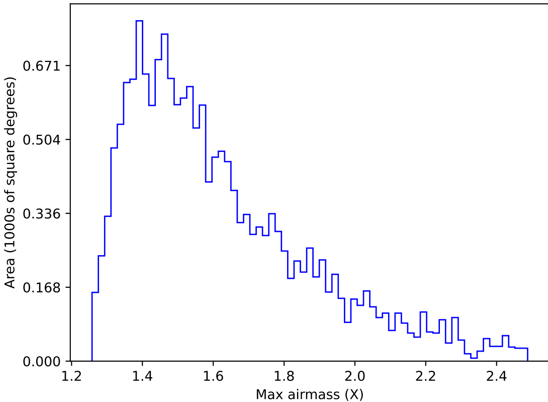
noroll_mjdp180_v3.4_10yrs WFD u band: Max airmass
