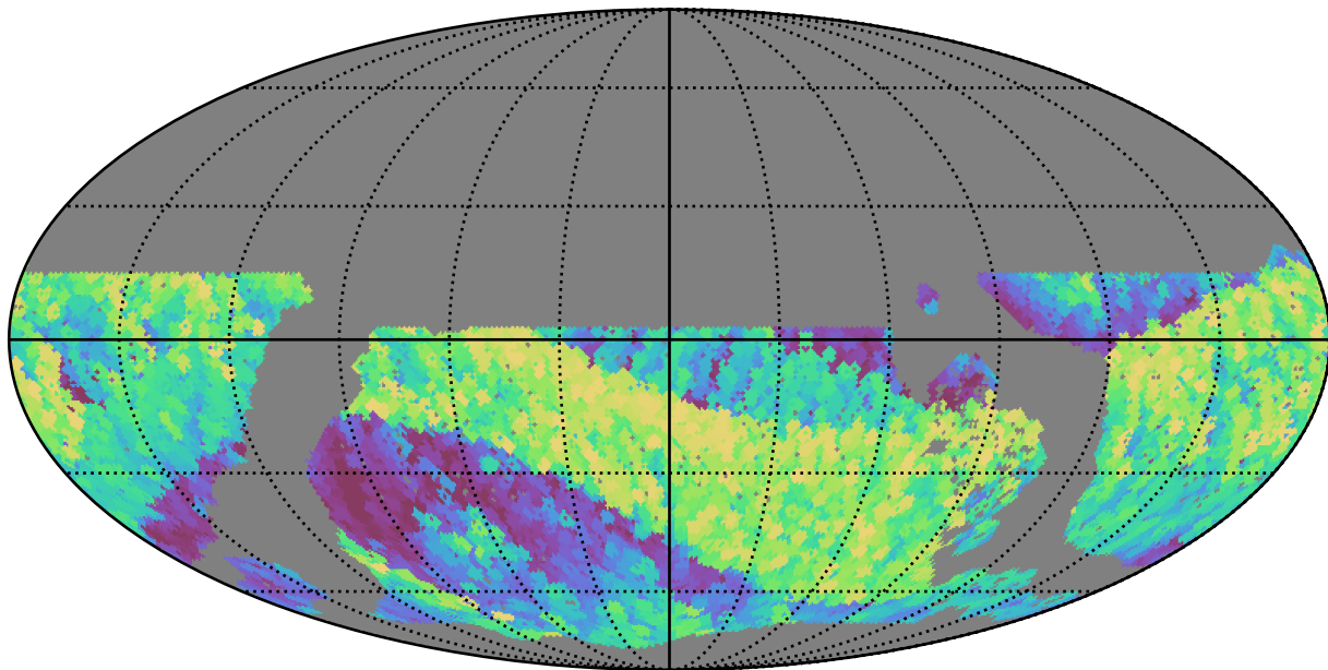
noroll_mjdp180_v3.4_10yrs WFD i band: Max airmass
