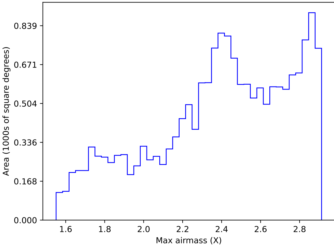
noroll_mjdp180_v3.4_10yrs WFD i band: Max airmass
