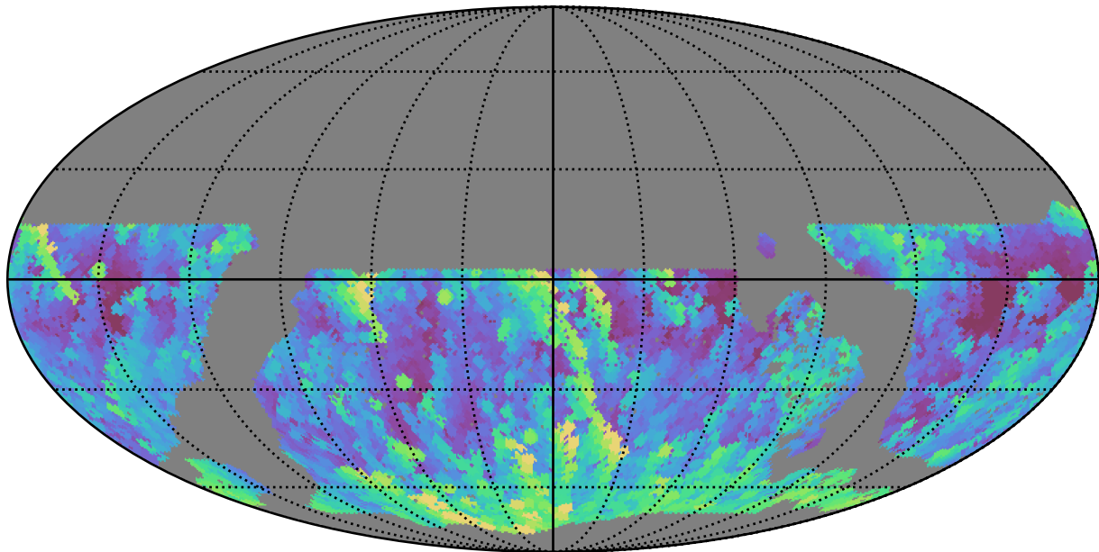
noroll_mjdp180_v3.4_10yrs WFD g band: Max airmass
