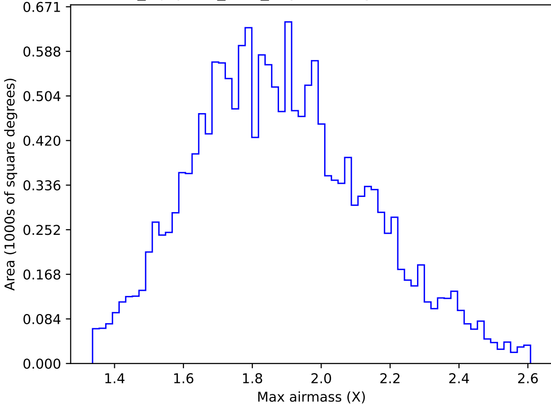
noroll_mjdp180_v3.4_10yrs WFD g band: Max airmass
