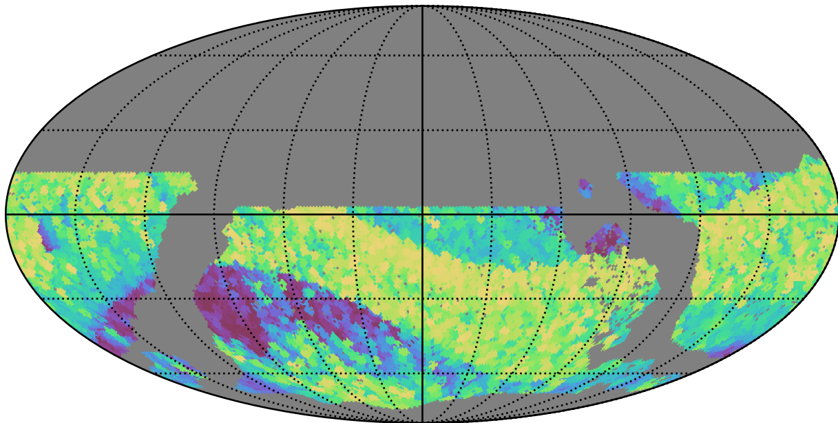
noroll_mjdp180_v3.4_10yrs WFD all bands: Max airmass
