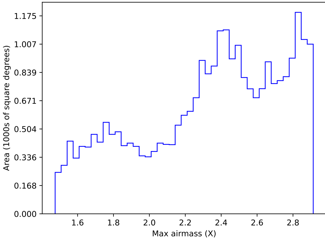
noroll_mjdp180_v3.4_10yrs All sky z band: Max airmass
