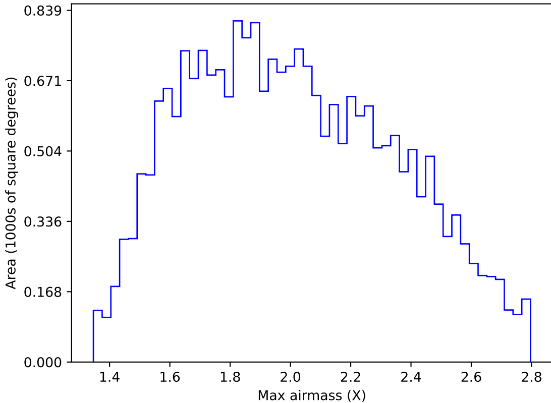
noroll_mjdp180_v3.4_10yrs All sky y band: Max airmass
