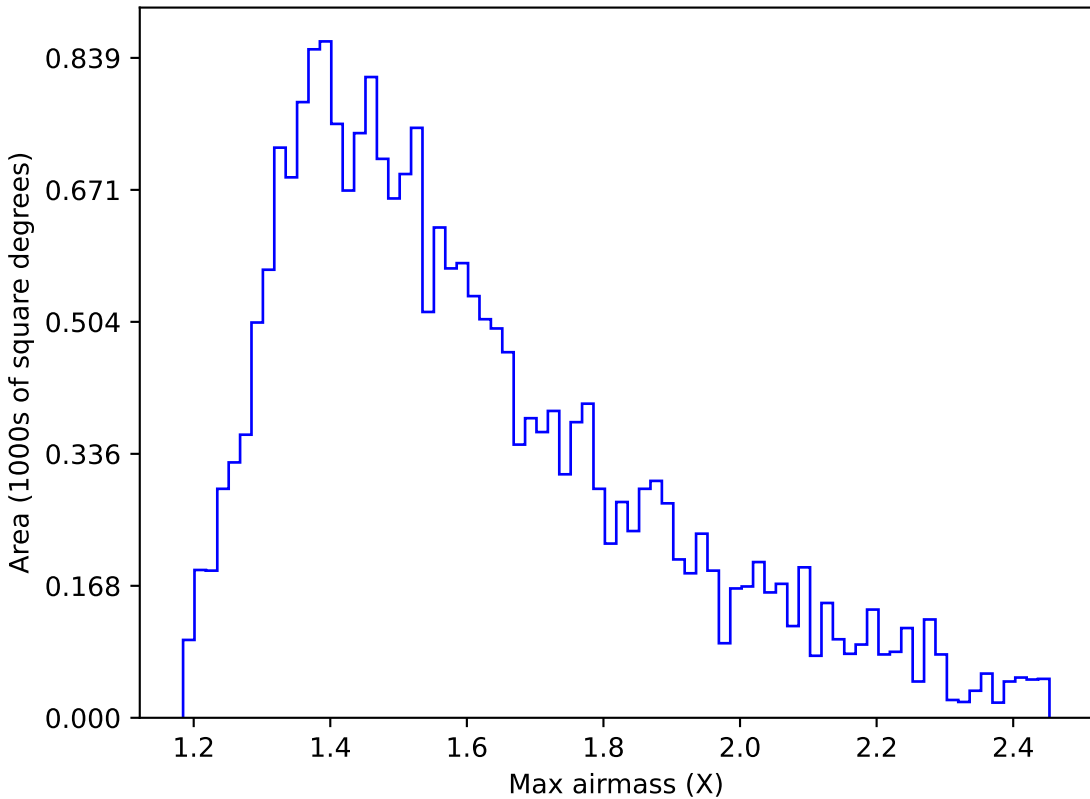
noroll_mjdp180_v3.4_10yrs All sky u band: Max airmass
