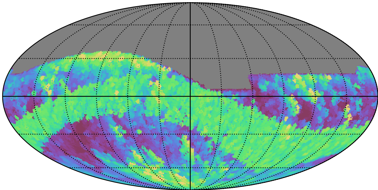
noroll_mjdp180_v3.4_10yrs All sky r band: Max airmass
