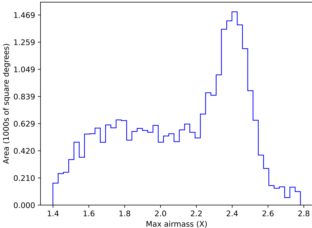
noroll_mjdp180_v3.4_10yrs All sky r band: Max airmass
