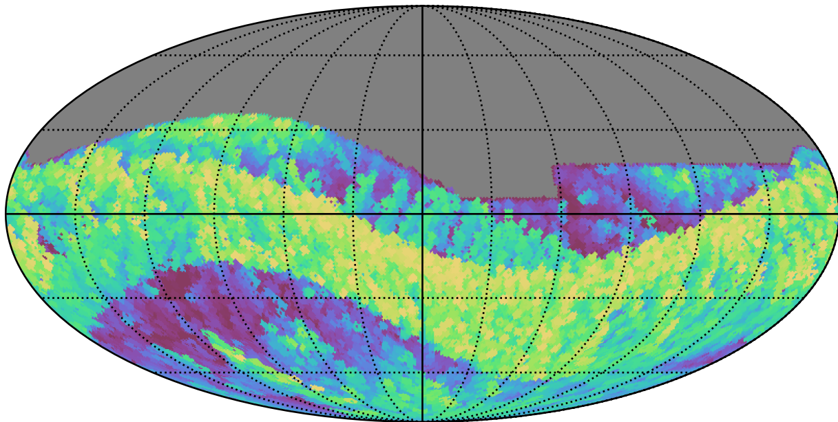
noroll_mjdp180_v3.4_10yrs All sky i band: Max airmass
