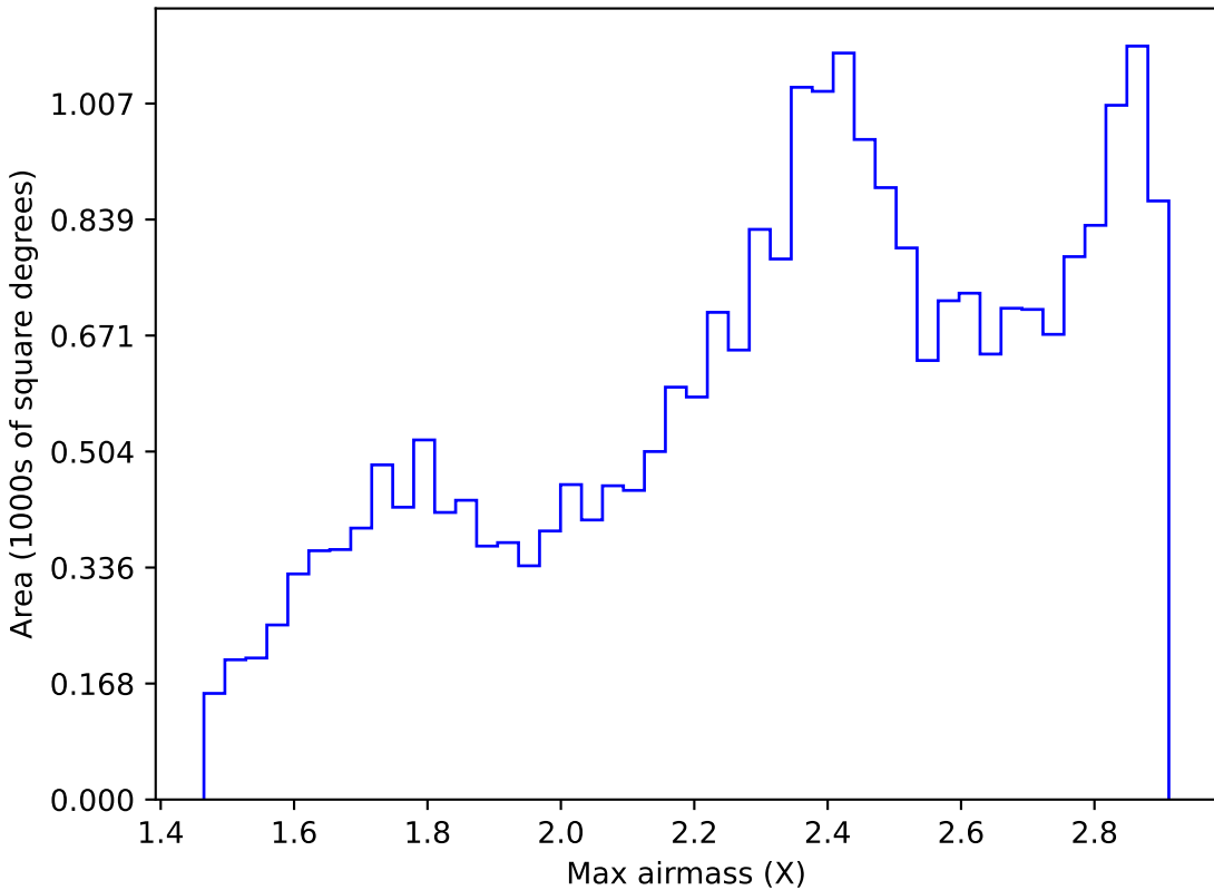
noroll_mjdp180_v3.4_10yrs All sky i band: Max airmass
