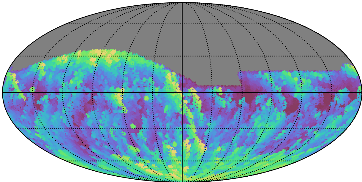
noroll_mjdp180_v3.4_10yrs All sky g band: Max airmass
