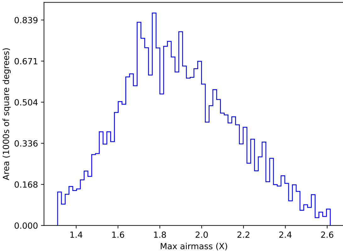
noroll_mjdp180_v3.4_10yrs All sky g band: Max airmass
