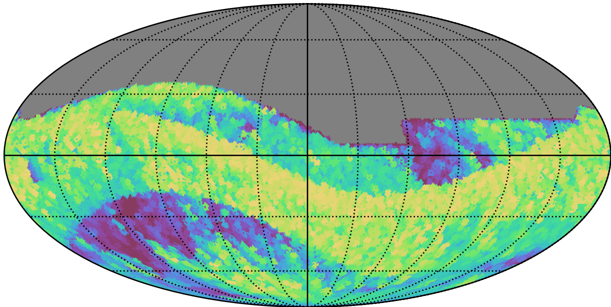
noroll_mjdp180_v3.4_10yrs All sky all bands: Max airmass
