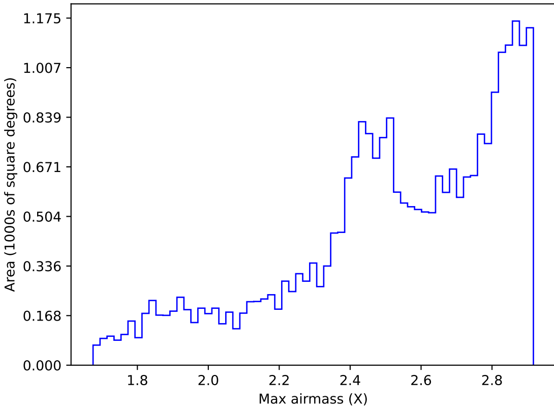
noroll_mjdp180_v3.4_10yrs All sky all bands: Max airmass
