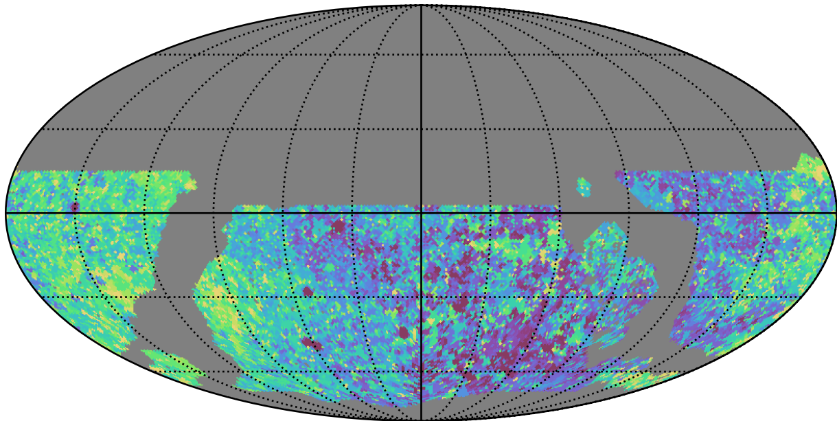
noroll_mjdp180_v3.4_10yrs WFD z band: Max Inter-Night Gap
