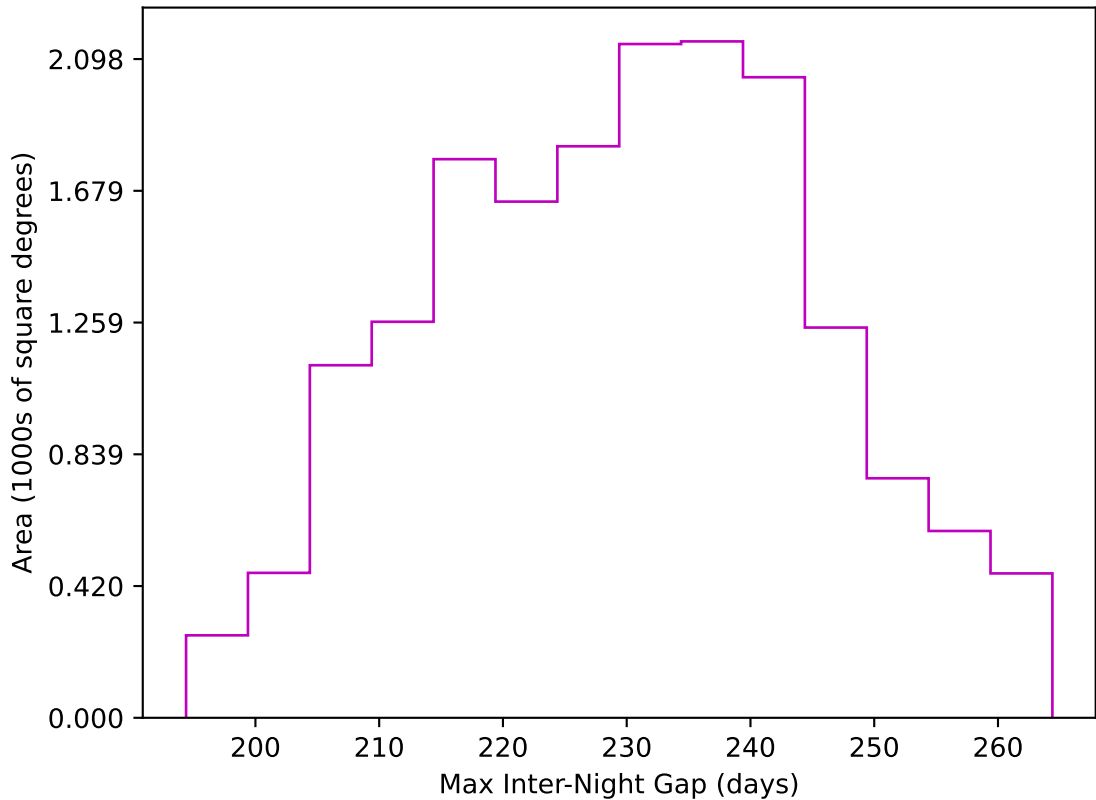
noroll_mjdp180_v3.4_10yrs WFD z band: Max Inter-Night Gap
