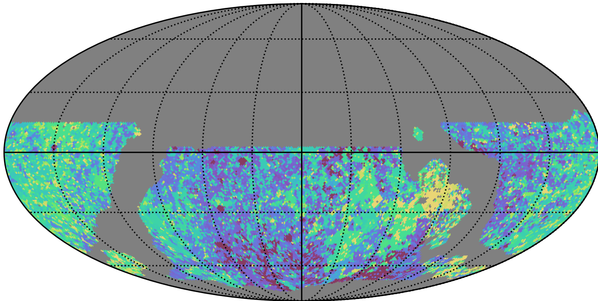
noroll_mjdp180_v3.4_10yrs WFD y band: Max Inter-Night Gap
