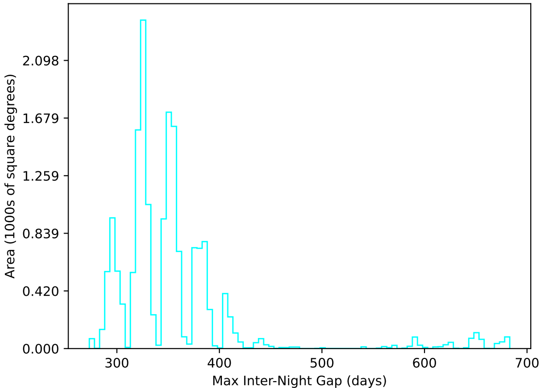
noroll_mjdp180_v3.4_10yrs WFD u band: Max Inter-Night Gap
