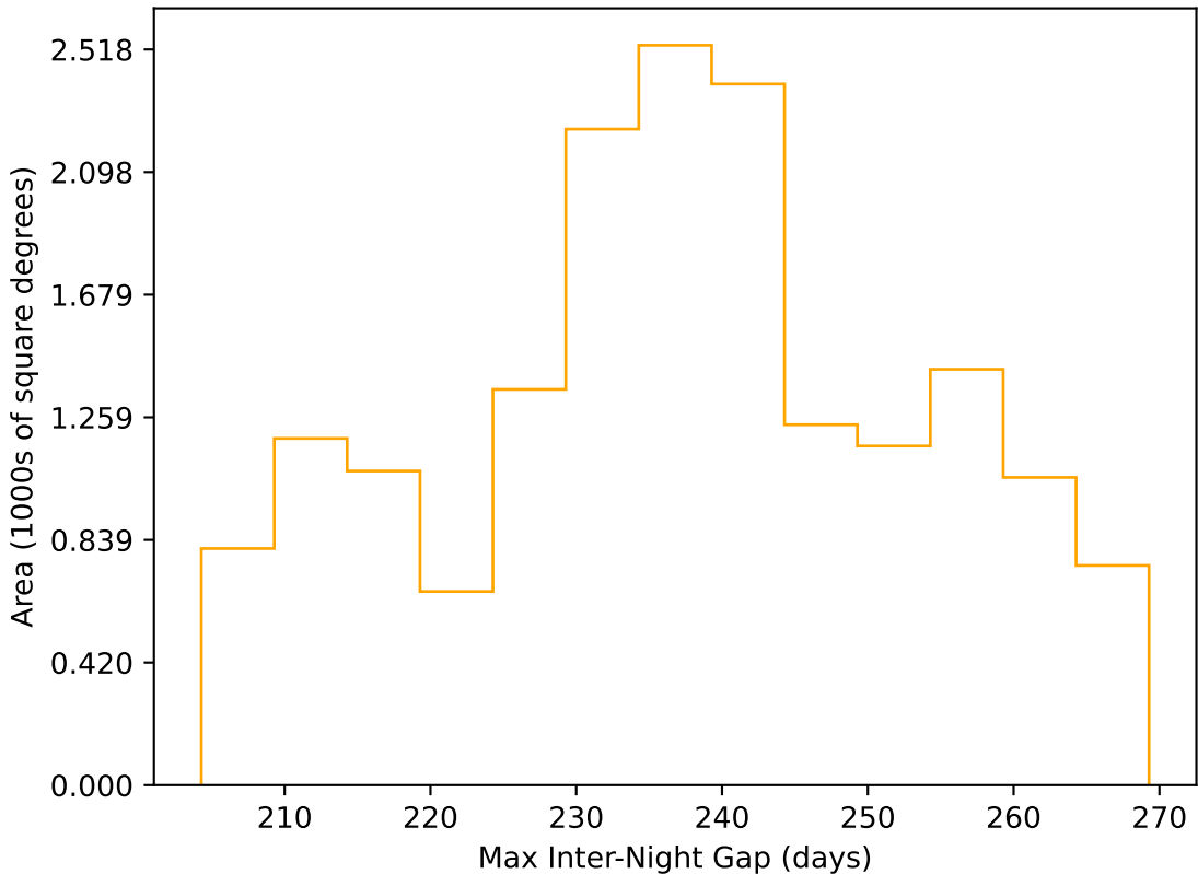
noroll_mjdp180_v3.4_10yrs WFD r band: Max Inter-Night Gap
