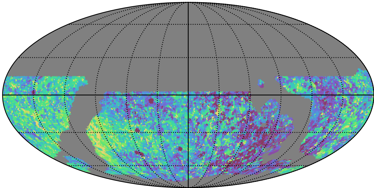
noroll_mjdp180_v3.4_10yrs WFD i band: Max Inter-Night Gap
