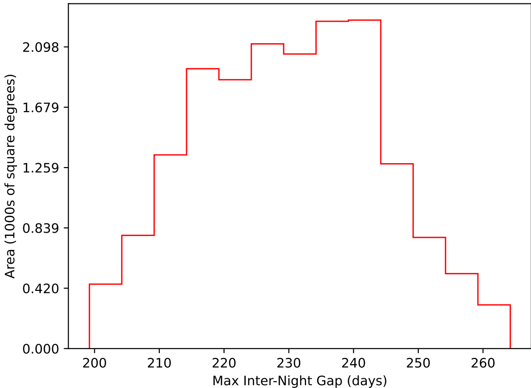
noroll_mjdp180_v3.4_10yrs WFD i band: Max Inter-Night Gap
