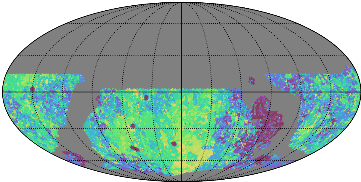
noroll_mjdp180_v3.4_10yrs WFD g band: Max Inter-Night Gap
