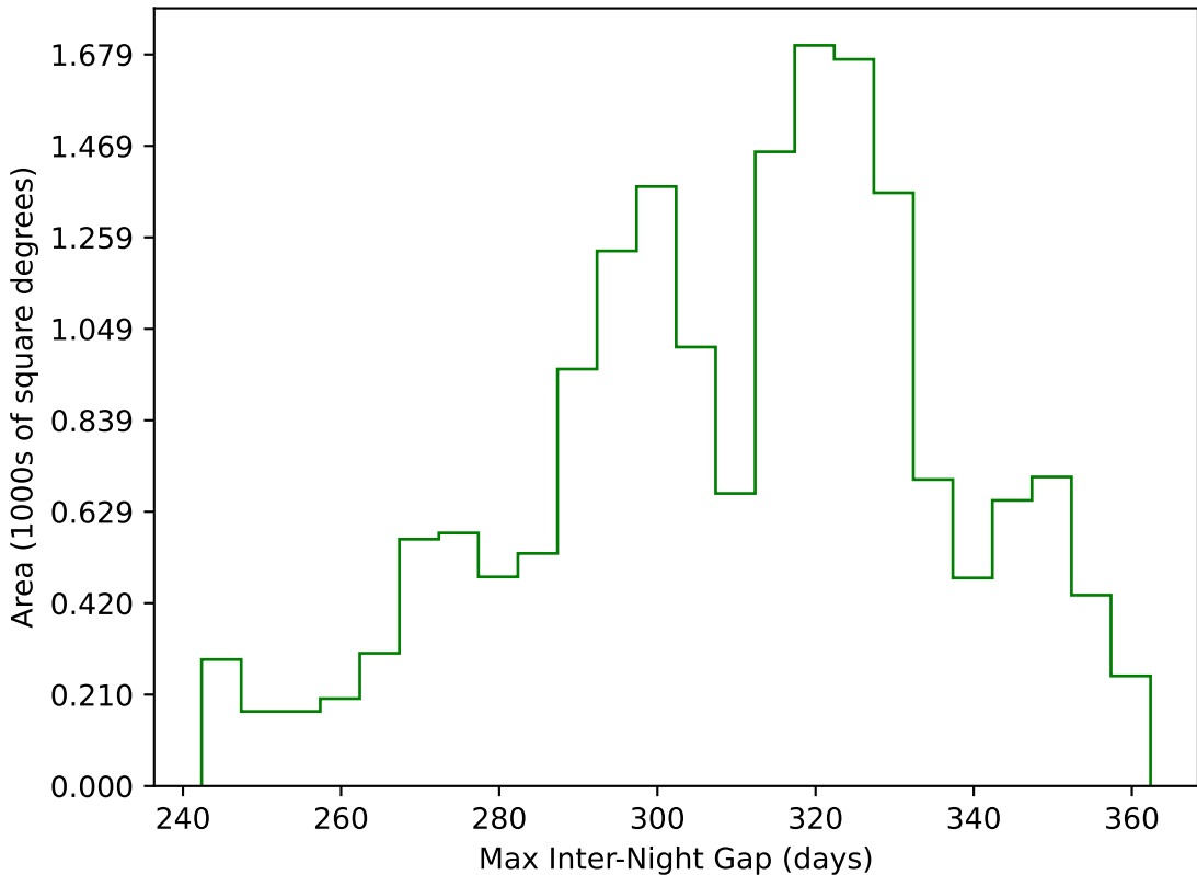
noroll_mjdp180_v3.4_10yrs WFD g band: Max Inter-Night Gap
