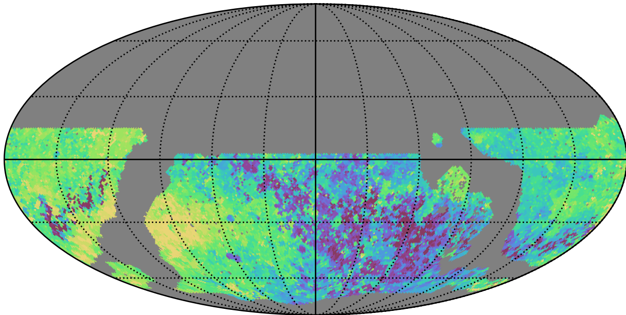
noroll_mjdp180_v3.4_10yrs WFD all bands: Max Inter-Night Gap
