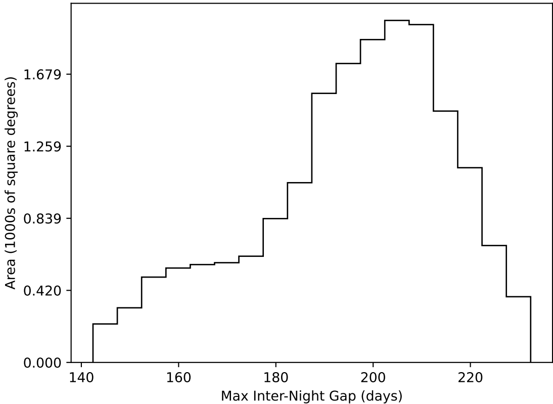
noroll_mjdp180_v3.4_10yrs WFD all bands: Max Inter-Night Gap
