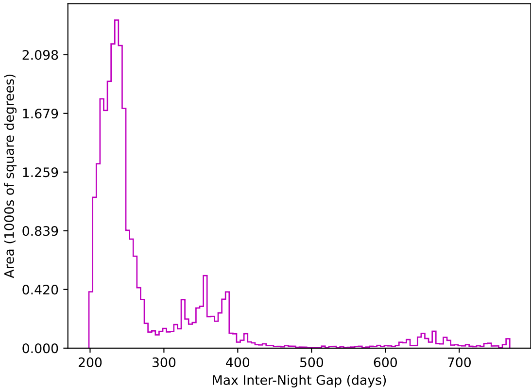
noroll_mjdp180_v3.4_10yrs All sky z band: Max Inter-Night Gap
