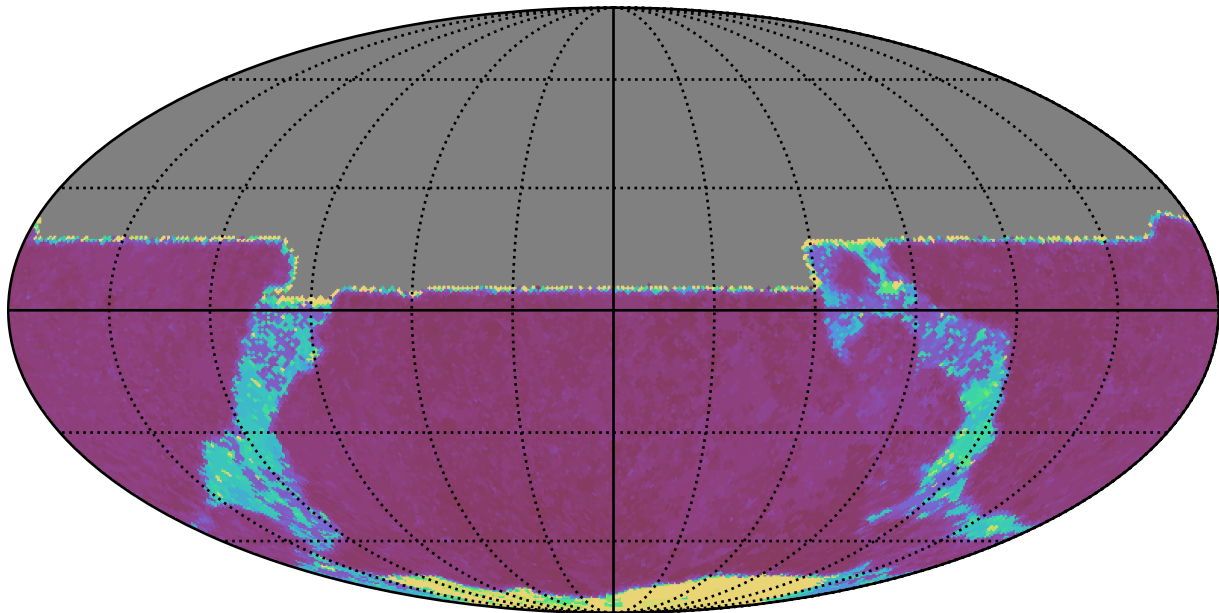
noroll_mjdp180_v3.4_10yrs All sky y band: Max Inter-Night Gap
