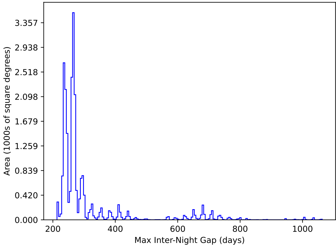
noroll_mjdp180_v3.4_10yrs All sky y band: Max Inter-Night Gap
