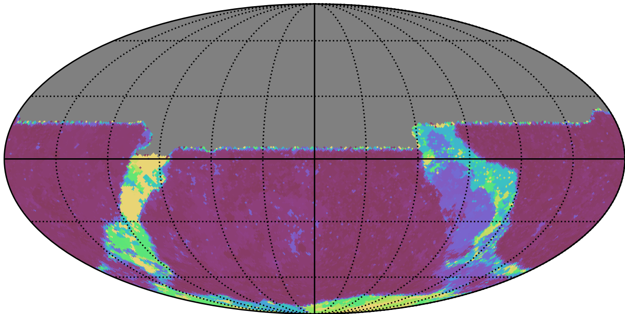
noroll_mjdp180_v3.4_10yrs All sky u band: Max Inter-Night Gap
