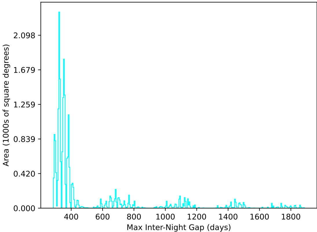
noroll_mjdp180_v3.4_10yrs All sky u band: Max Inter-Night Gap
