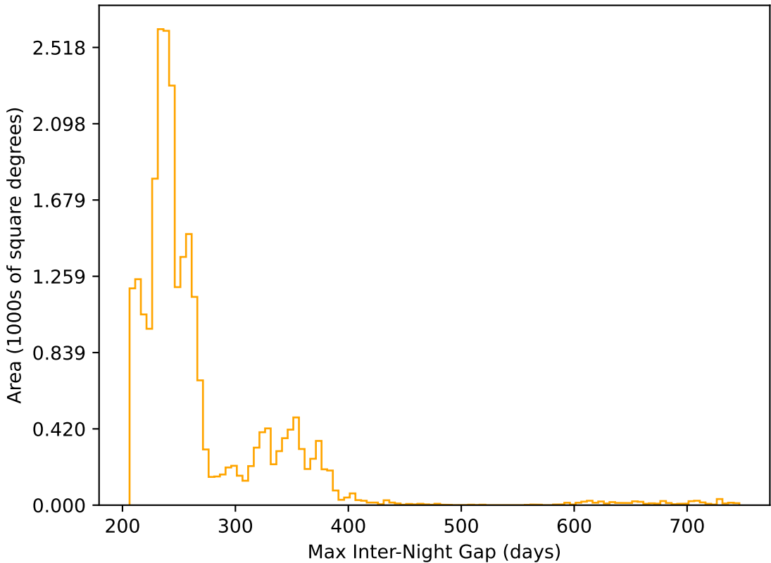
noroll_mjdp180_v3.4_10yrs All sky r band: Max Inter-Night Gap
