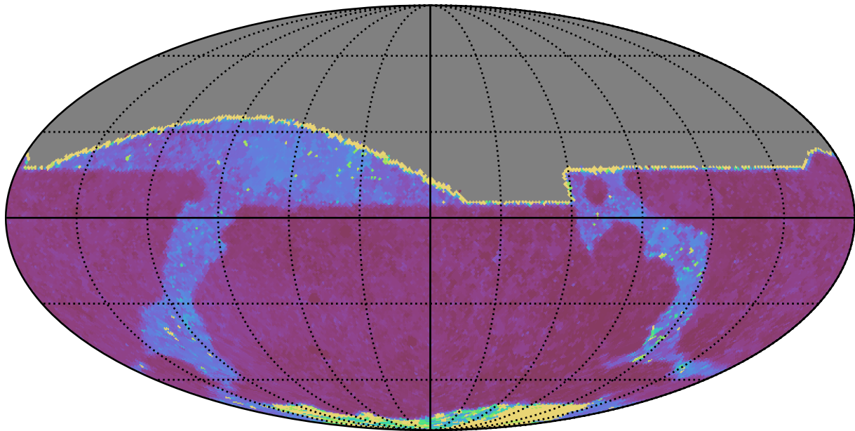
noroll_mjdp180_v3.4_10yrs All sky i band: Max Inter-Night Gap
